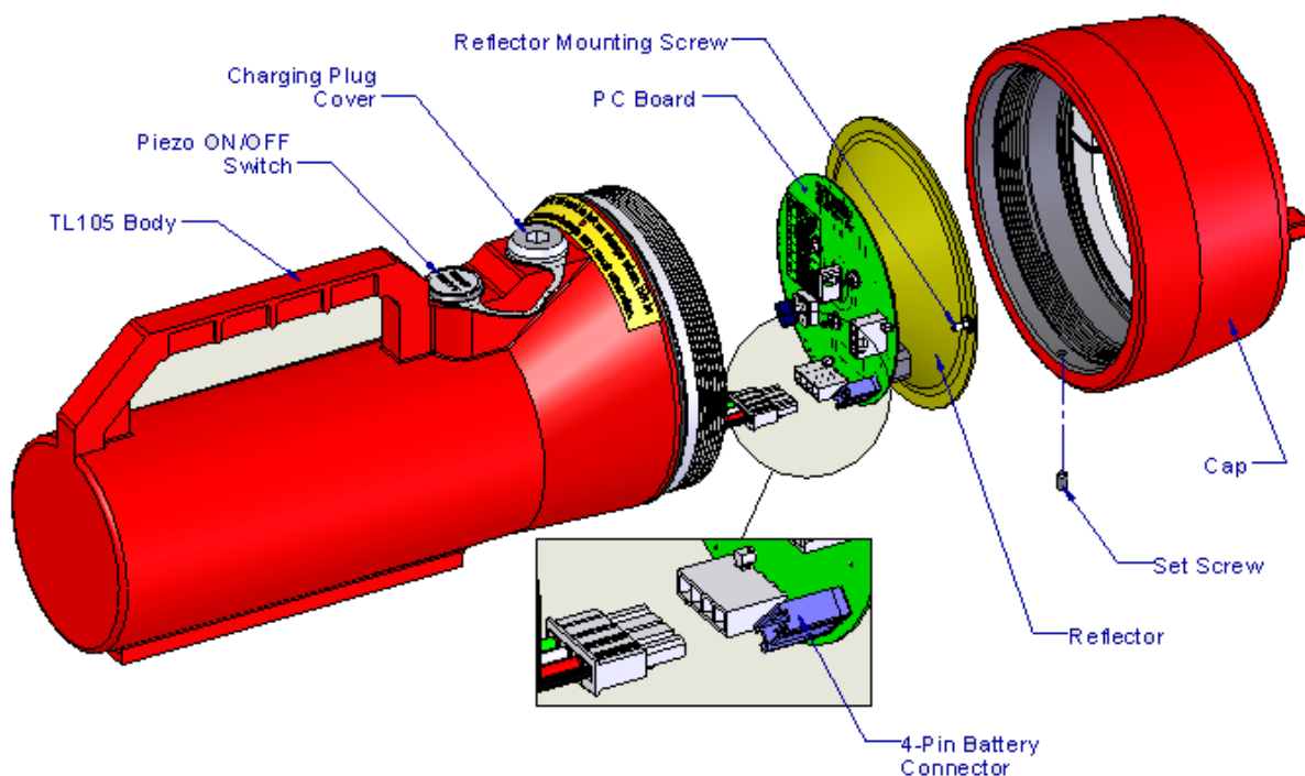
Figure 2: TL105 Battery Connection
